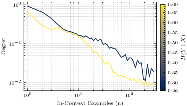
In-Context Learning Regret for Qwen-2.5 (32B)
